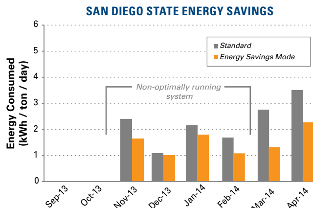
Figure 2: Energy savings from the CATALYST system in Energy Savings Mode compared to Standard Mode (Standard Mode shows similar performance before the CATALYST retrofit)
