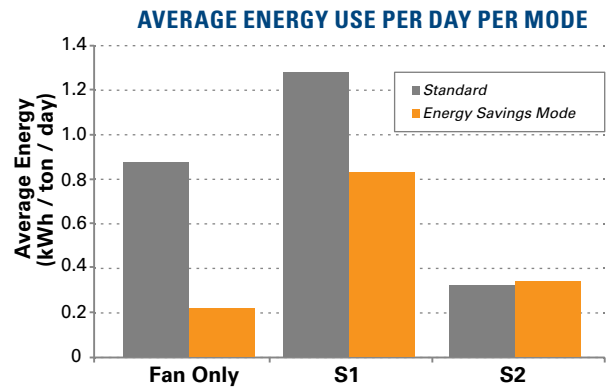
Figure 3: Energy consumption at CSU Long Beach in various modes of operation
