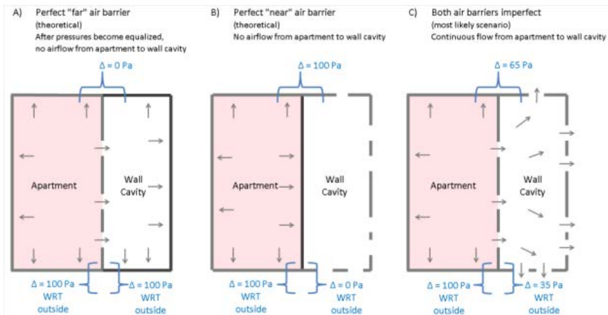
Figure 13. Locations of air barriers in walls
