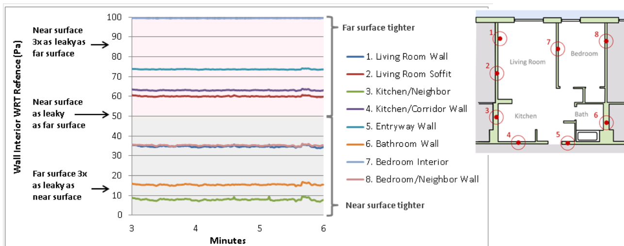
Figure 27. Leakage characteristics of walls before sealing
