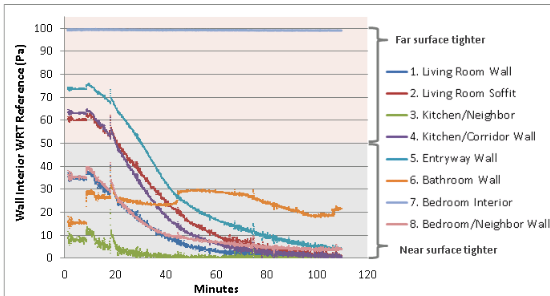
Figure 30. Pressures in walls during sealing
