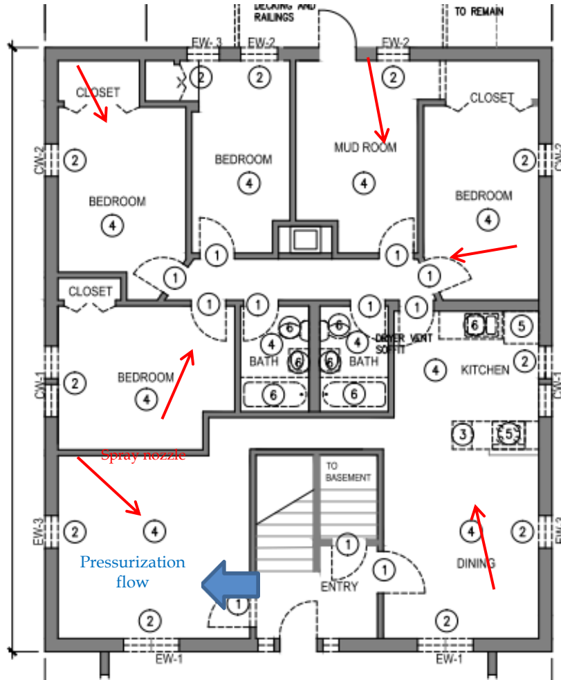
Figure 36: Unit 2 floor plan with nozzle and fan locations
