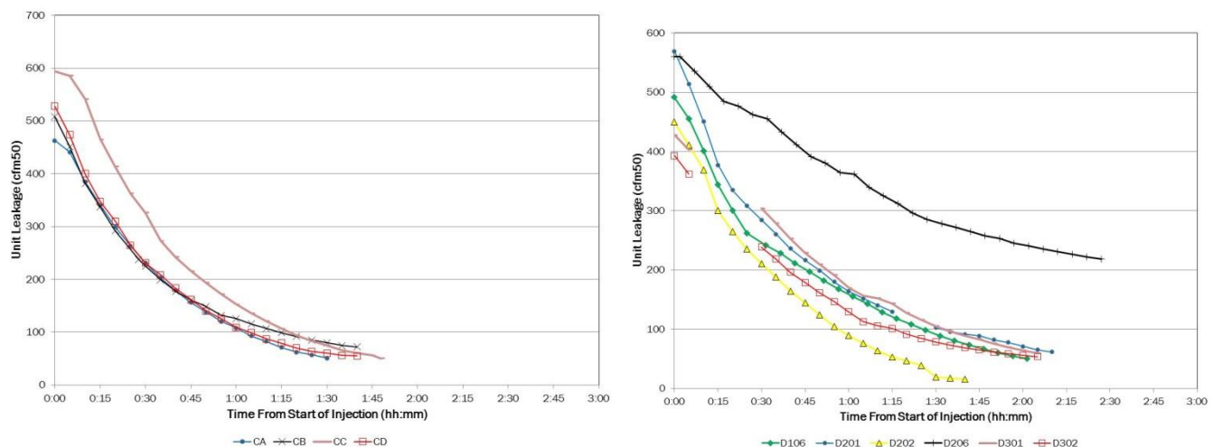
Figure 4. Variation in unit leakage (cfm50) through aerosol sealing process for units in new construction building C (left) and existing building D (right)
