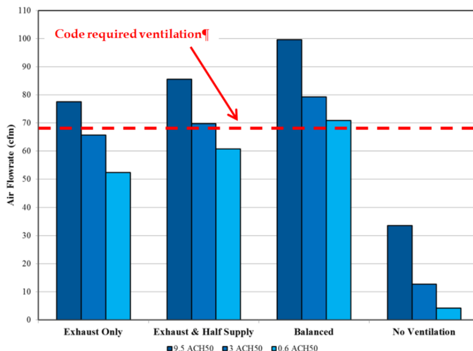
Figure 48: Modeled annual average ventilation flowrate for three tightness scenarios
