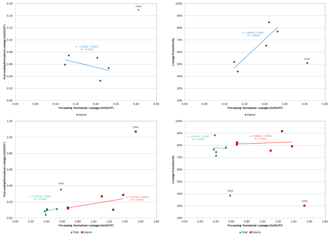
Figure 40: Pre and post sealing unit leakage and percent reduction for existing units
