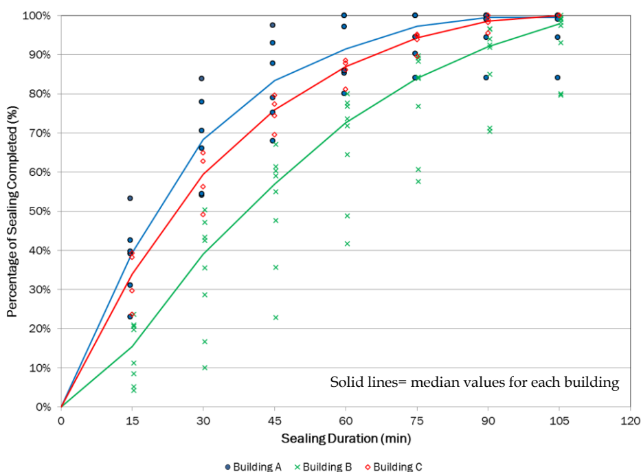
Figure 30: Percent of sealing completed over time
