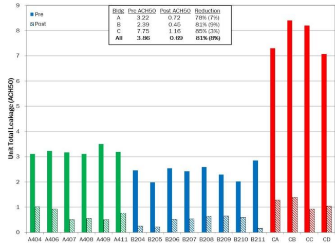
Figure 5. Pre and post sealing unit leakage and percent reduction for new construction units
