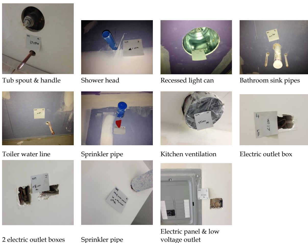
Figure 33: Photos of unit A409 sites with pre-sealing measured leakage
