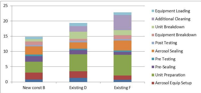
Figure 7. Average task labor times in person-hours per unit for sealed units in three existing buildings
