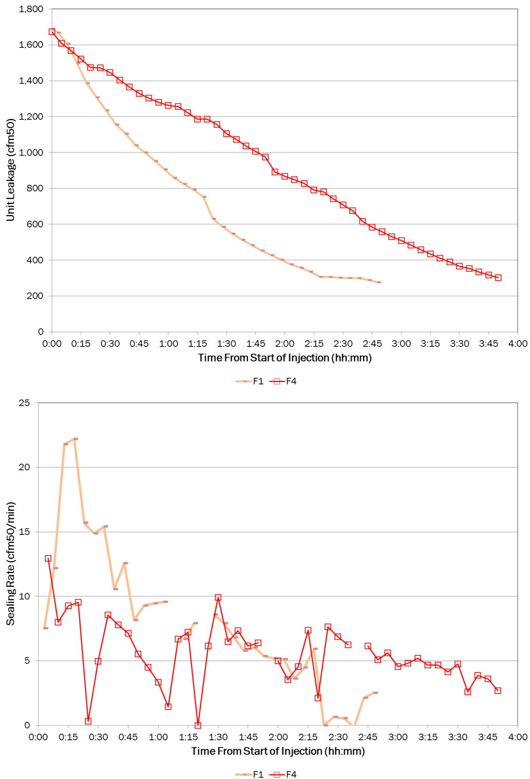
Figure 37: Variation in unit leakage (top) and sealing rate (bottom): Building F
