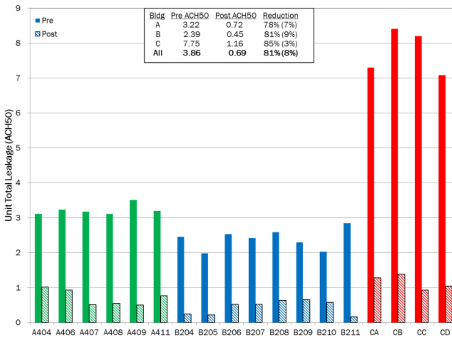
Figure 32: Pre and post sealing unit leakage and percent reduction for new construction units
