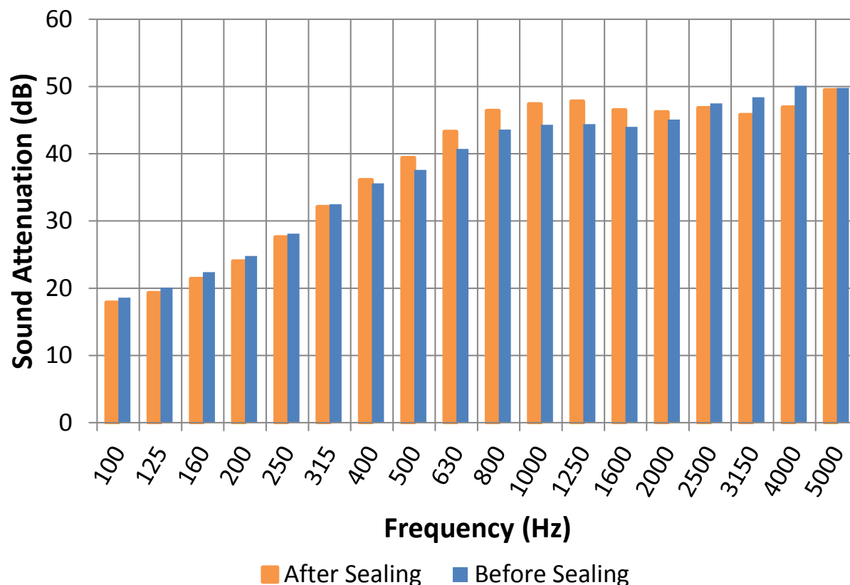
Figure 43: Sound attenuation across a wall before and after sealing with aerosol technology
