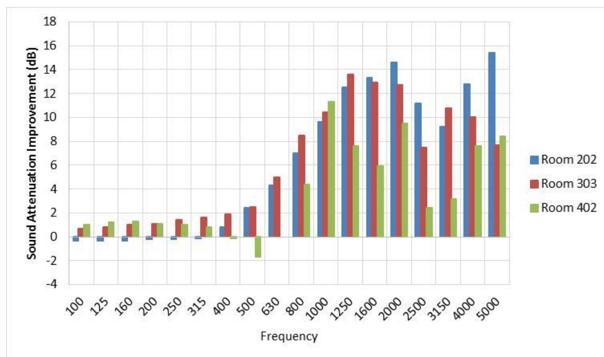
Figure 16: Sound attenuation results for three apartments sealed in Queens, NY
