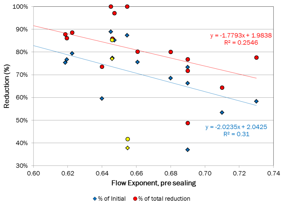
Figure 31: Variation of first hour sealing rate with leakage flow exponent
