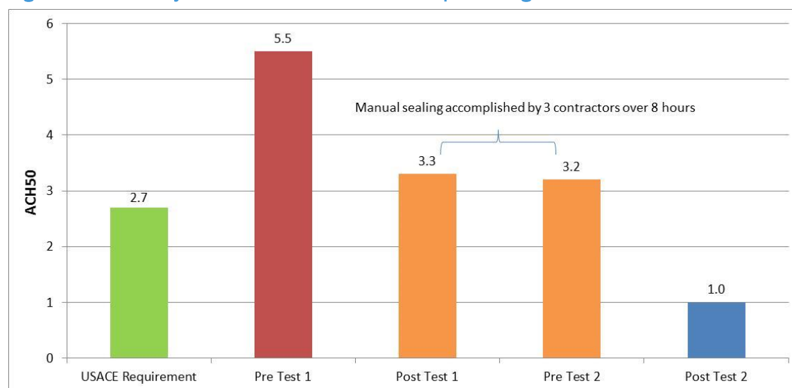
Figure 12: Summary of results from aerosol envelope sealing demonstration in Honda Smart Home
