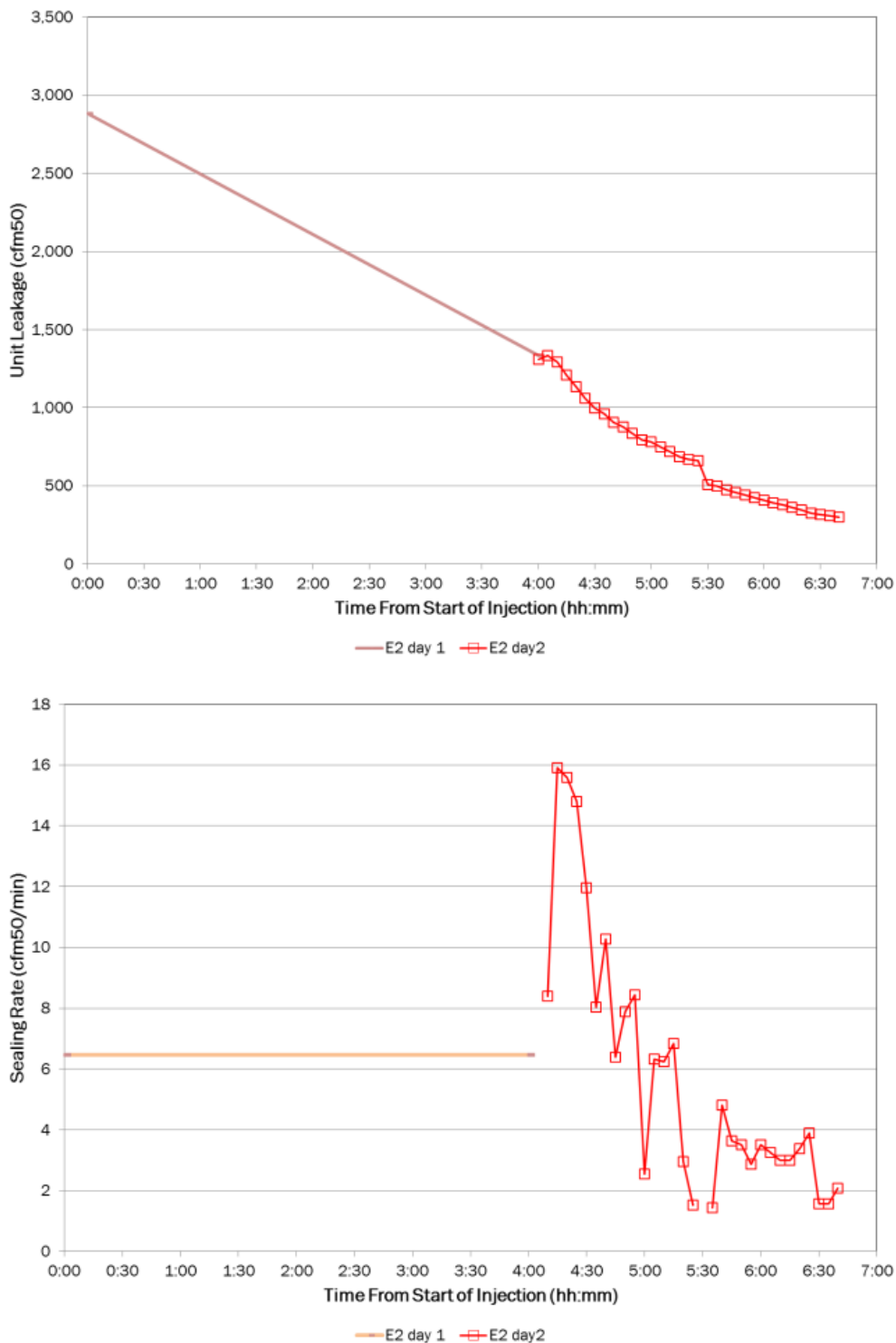
Figure 35: Variation in unit leakage (top) and sealing rate (bottom): Building E 16
