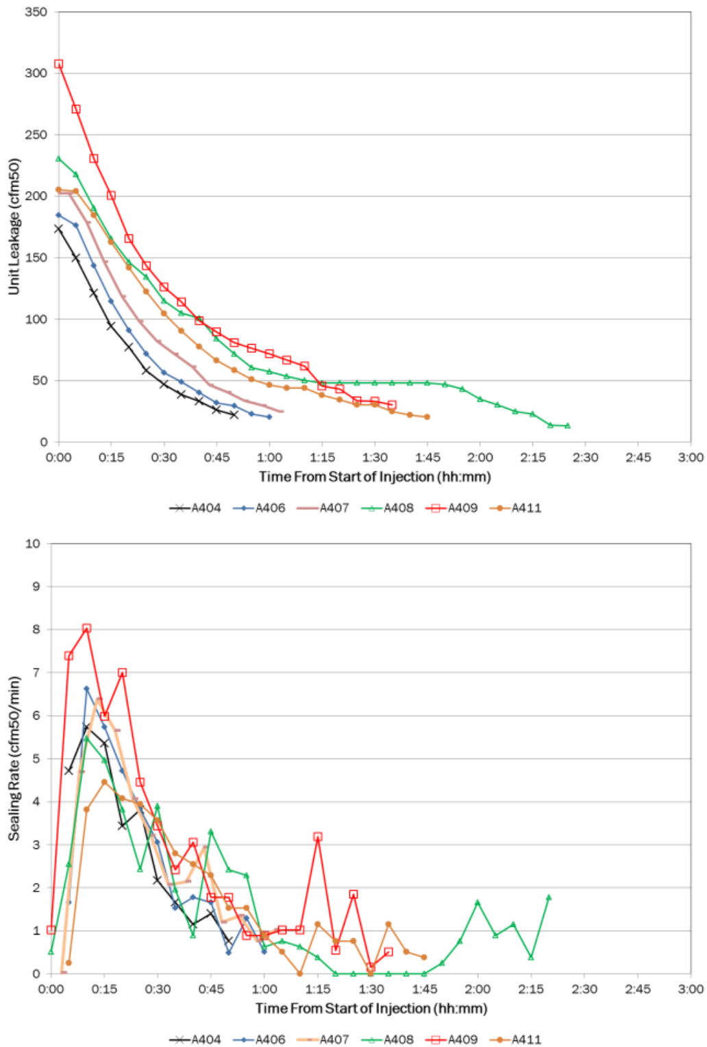
Figure 27: Variation in unit leakage (top) and sealing rate (bottom): Building A
