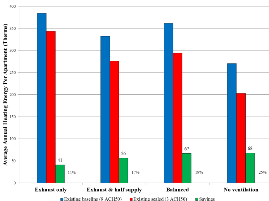
Figure 47: Modeled annual space heating energy use and savings for existing building units
