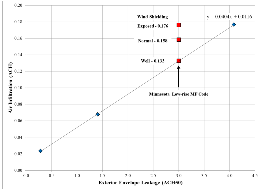
Figure 50: Modeled heating season air infiltration for three tightness scenarios and balanced ventilation
