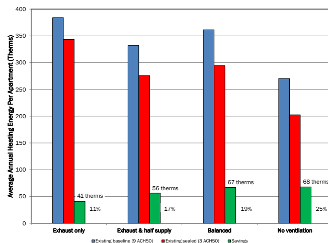
Figure 9. Modeled annual space heating energy use and savings for existing building units
