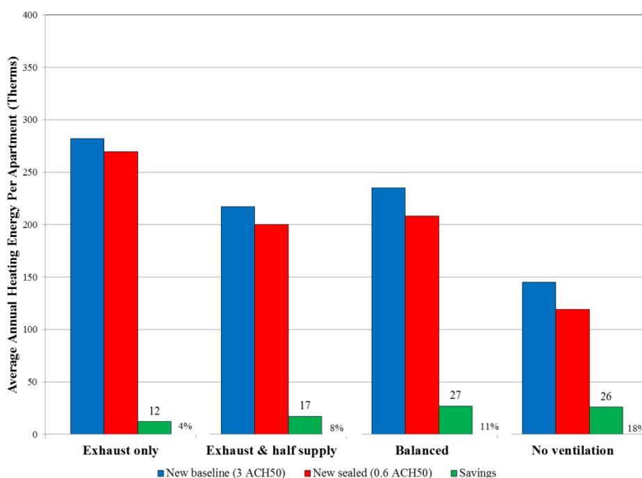
Figure 45: Modeled annual space heating energy use and savings for new construction units
