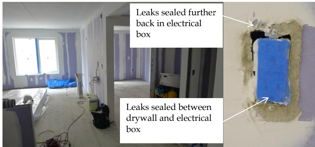
Figure 13: Photos of one apartment before being sealed and sealed electrical box
