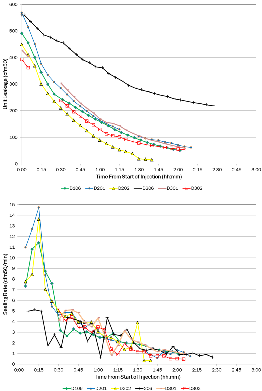
Figure 34: Variation in unit leakage (top) and sealing rate (bottom): Building D
