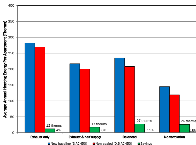
Figure 8. Modeled annual space heating energy use and savings for new construction units
