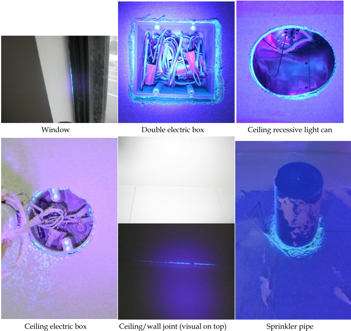
Figure 26: UV images of sealed air leaks
