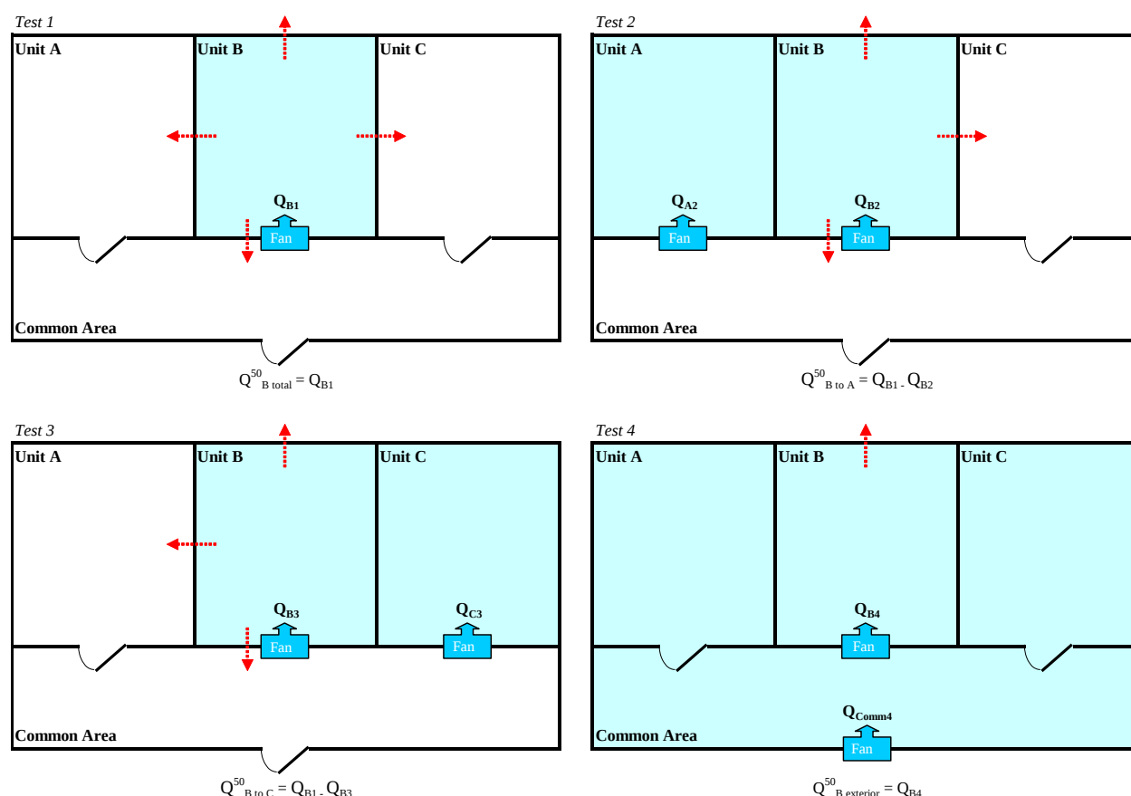
Figure 20: Guarded-zone test sequence for three unit apartment building
