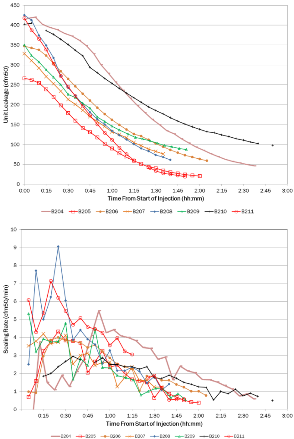
Figure 28: Variation in unit leakage (top) and sealing rate (bottom): Building B
