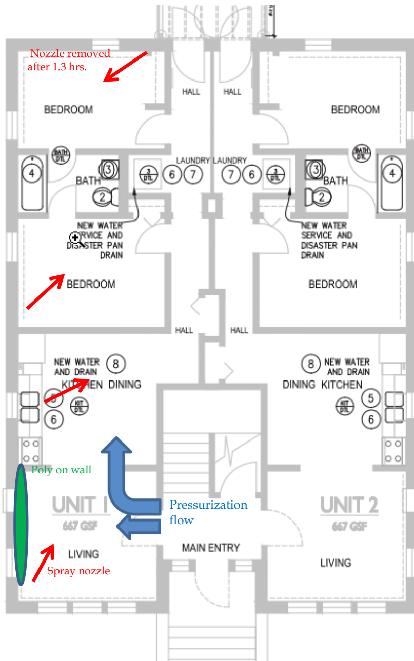
Figure 38: Unit 1 floor plan with nozzle and fan locations 17
