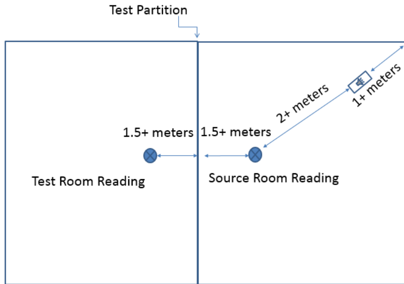
Figure 22: Sound Test Setup Diagram
