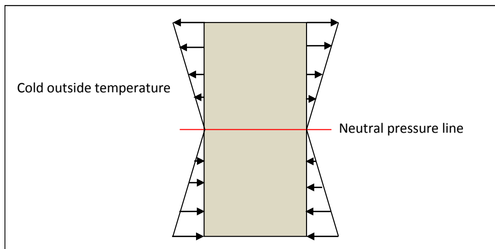
Figure 23: Illustration of stack effect during the heating season. Warm indoor air exits near the top of the building while make-up air enters from the bottom of the building
