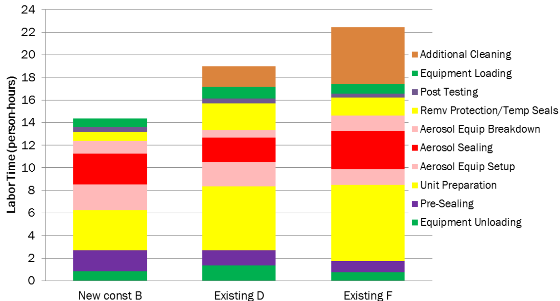
Figure 44: Breakdown of labor per unit in person-hours for 10 sealing tasks
