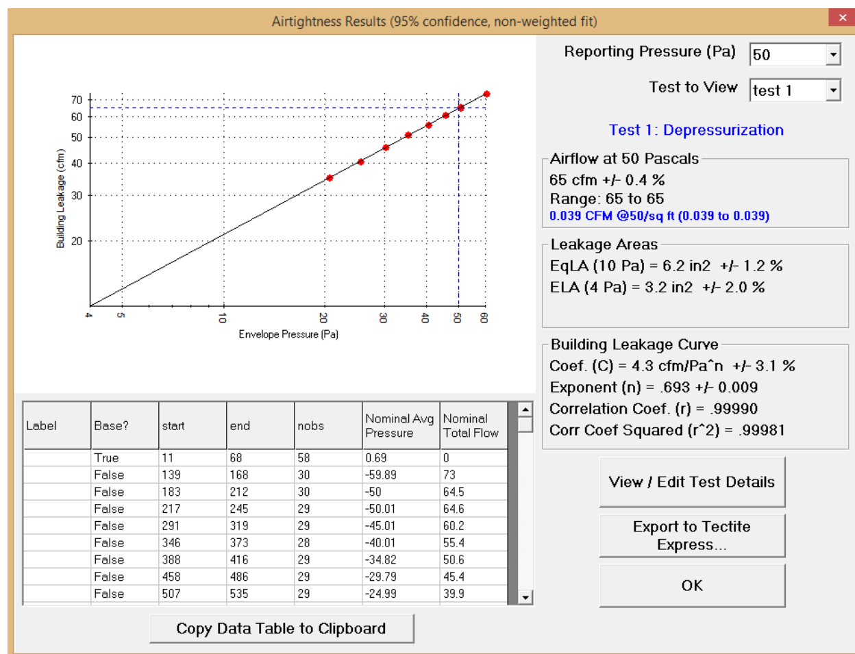
Figure 19: Regression analysis for a typical test
