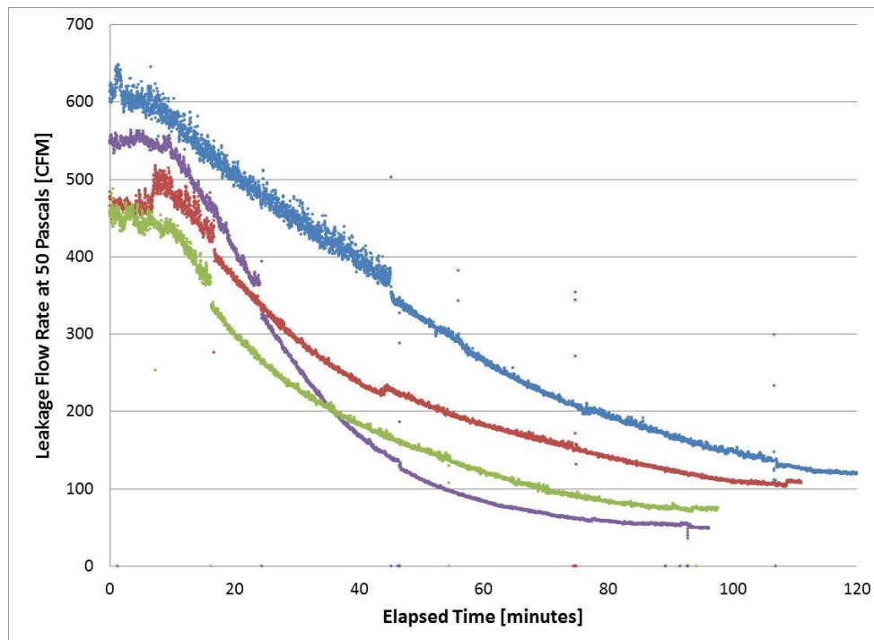
Figure 15: Sealing profiles for demonstration of aerosol sealing process on four apartments in Queens, NY
