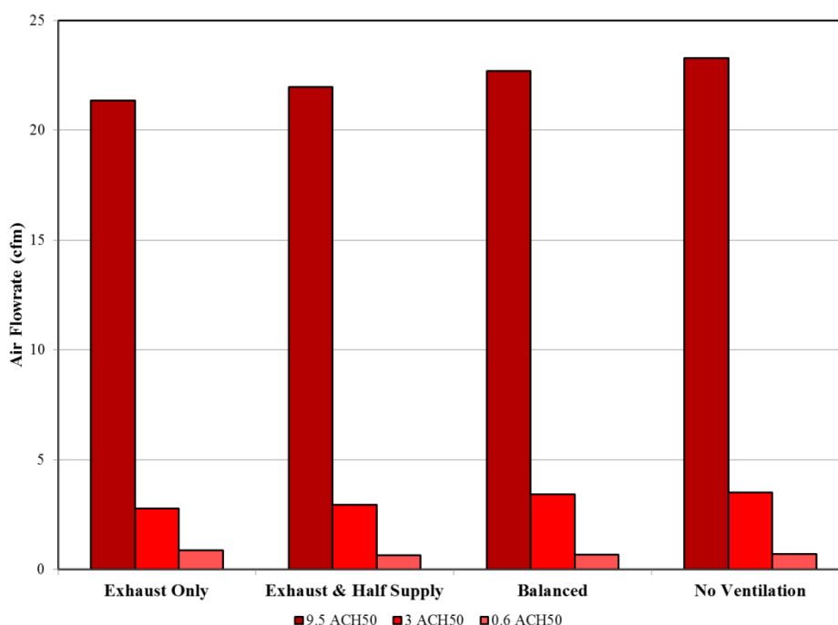
Figure 51: Modeled annual average flowrate from adjoining units
