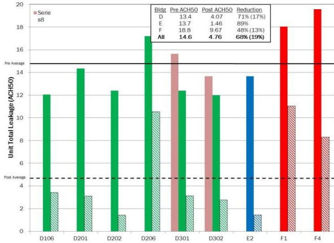
Figure 6. Pre and post sealing unit leakage and percent reduction for existing units
