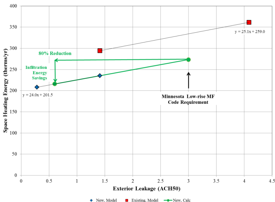
Figure 46: Annual space heating energy use for balanced ventilation
