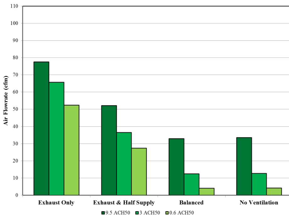
Figure 49: Modeled annual average air infiltration for three tightness scenarios
