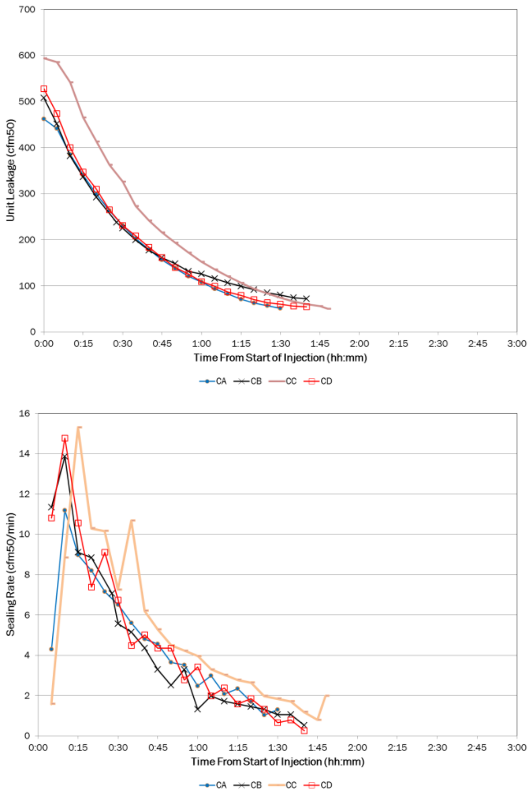
Figure 29: Variation in unit leakage (top) and sealing rate (bottom): Building C
