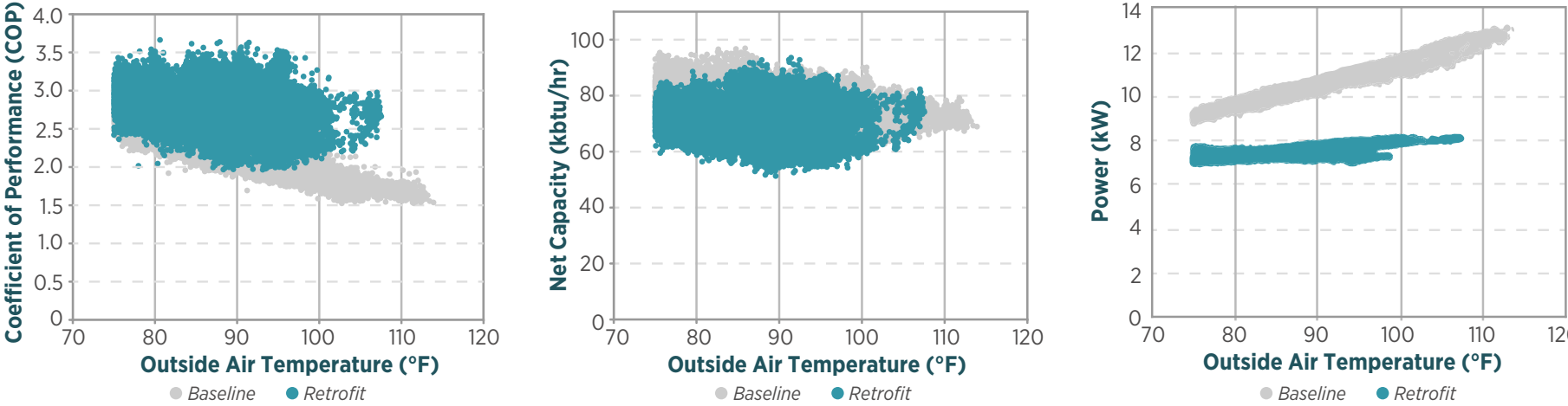
Performance graphs comparing the retrofit optimization package to the baseline RTU
