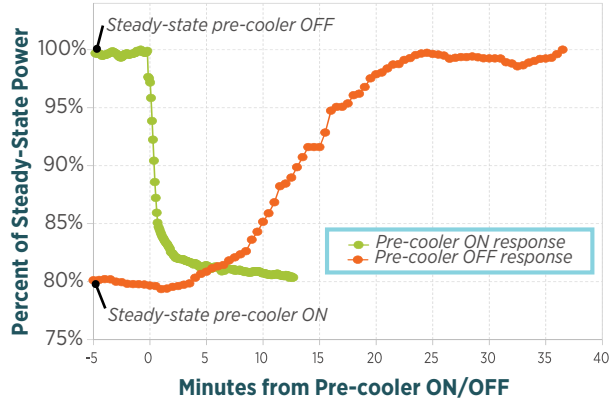
Field test of aggregate power usage of pre-coolers on/off based on OAT
