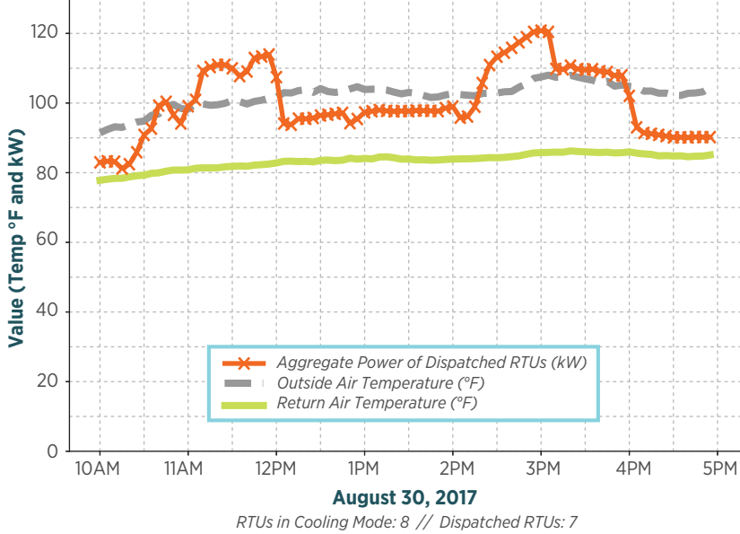
Response time of dispatchable pre-coolers
